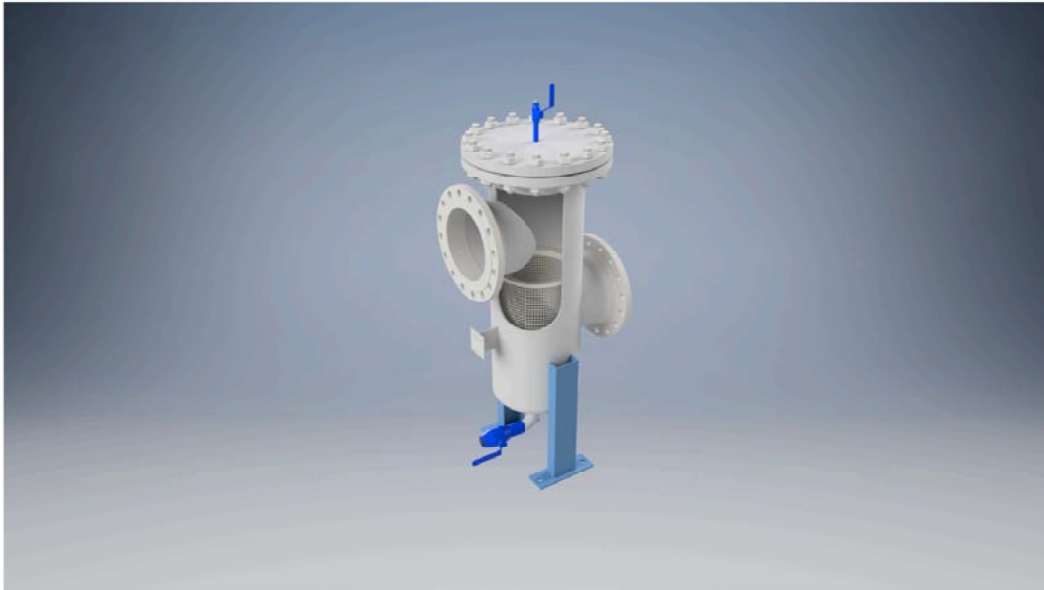
District heating filter dn 300
